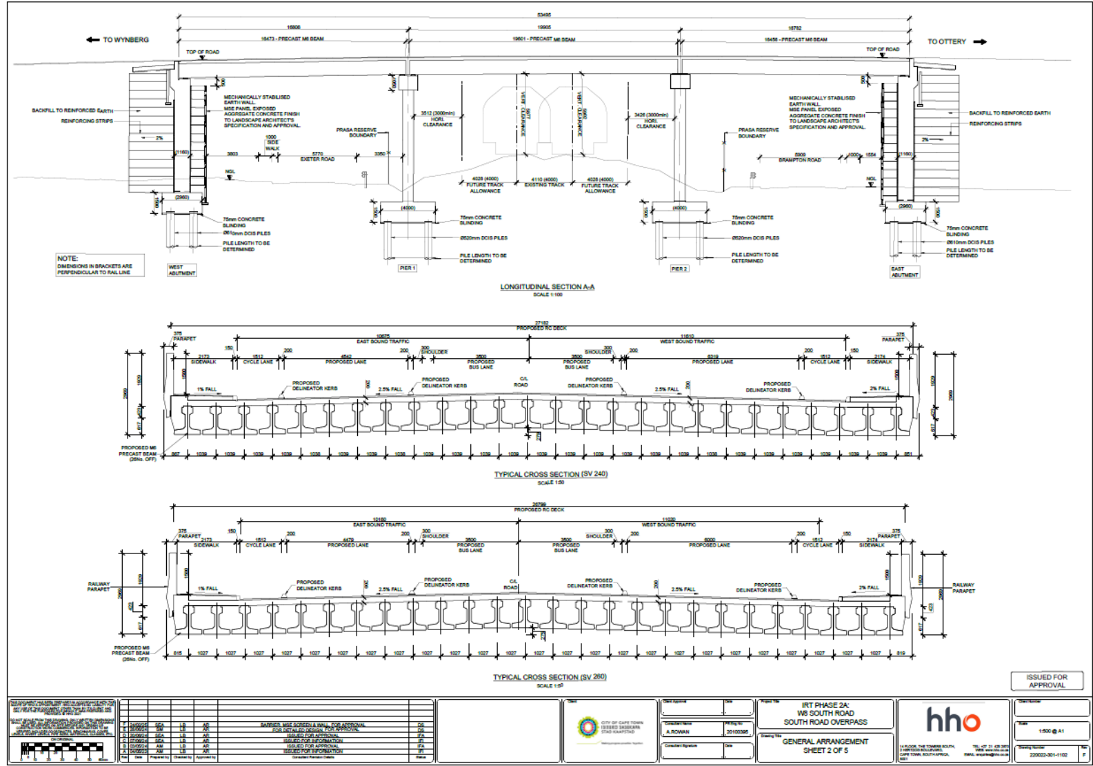
Figure 5: Typical cross section for bridge structure (rail overpass) (source: HHO, 2025)
